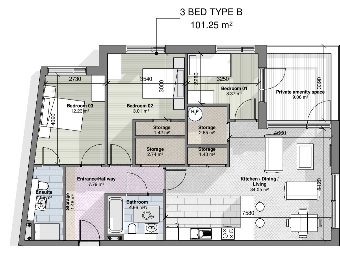
3 BEDROOM APARTMENT TYPE B 1 : 100
