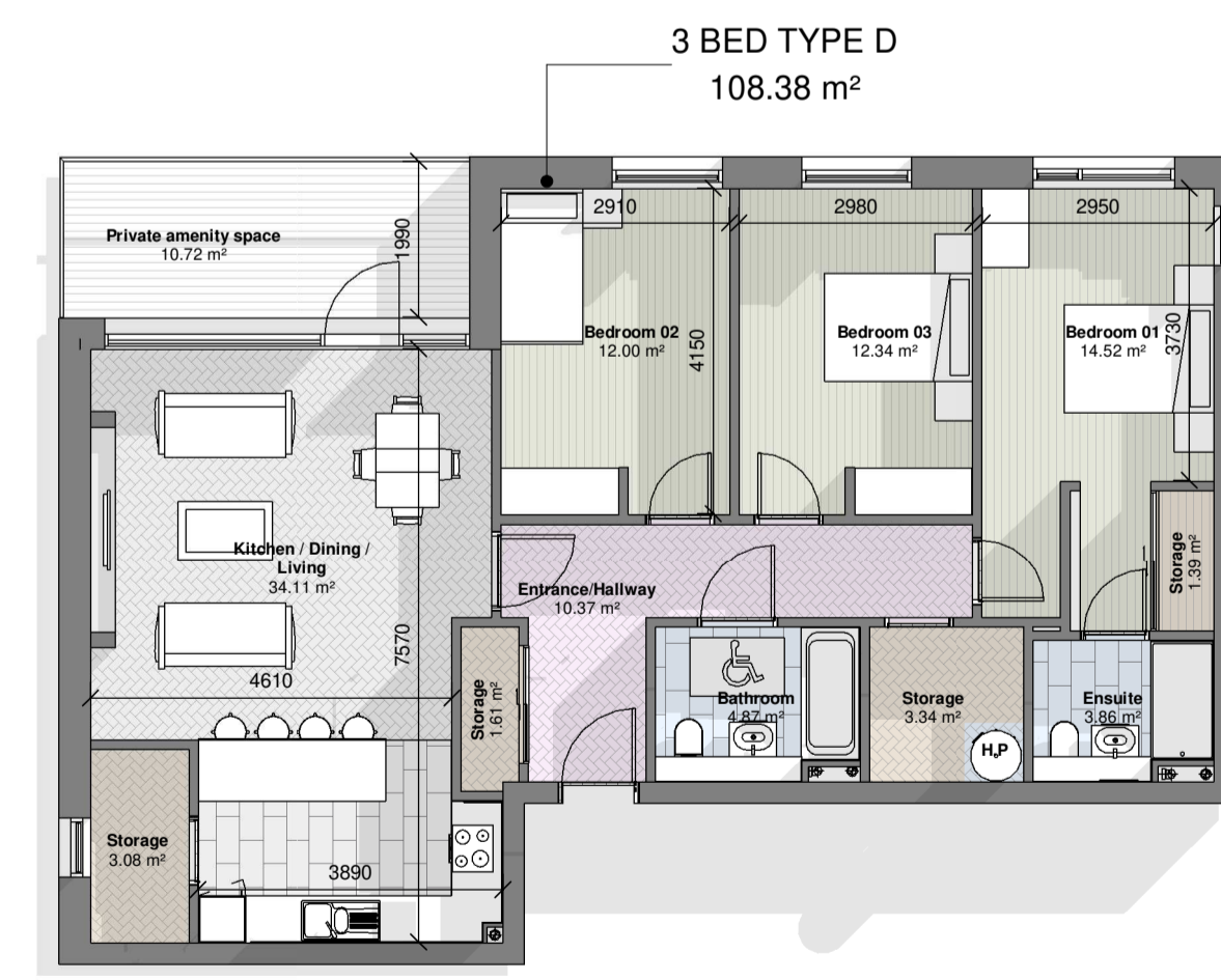
3 BEDROOM APARTMENT TYPE D 1 : 100
